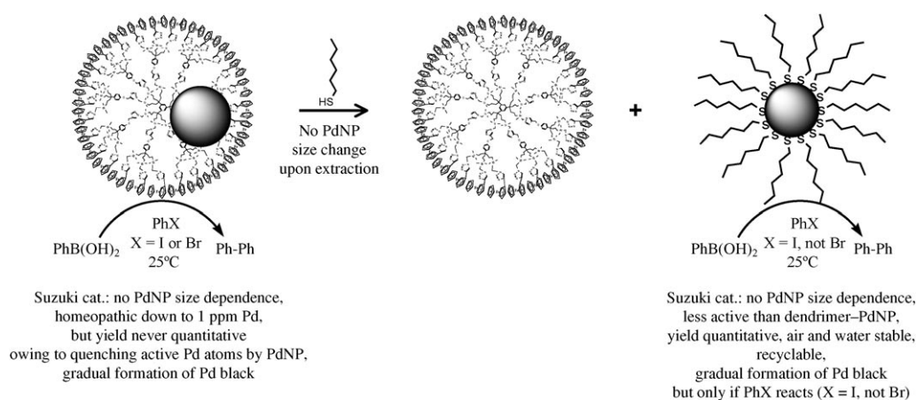
Scheme 2. Extraction of PdNPs from DSNs or DENs with hexanethiol without any change in the size of the PdNPs to produce air- and water-stable, catalytically active hexanethiolate PdNPs.
